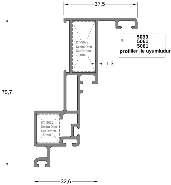
Kasa Profili Frame Profile
