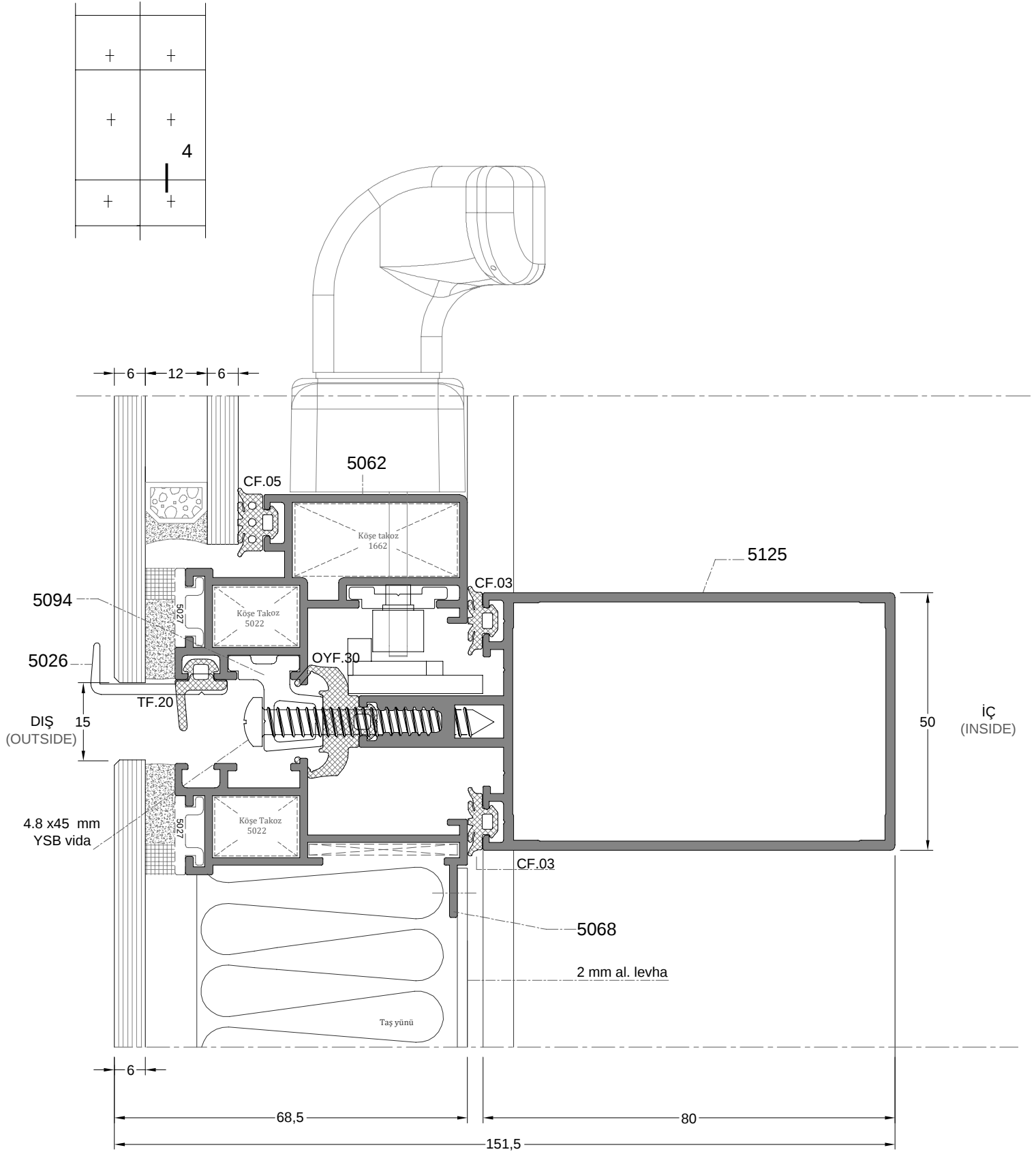
DETAY 4 DETAIL 4
