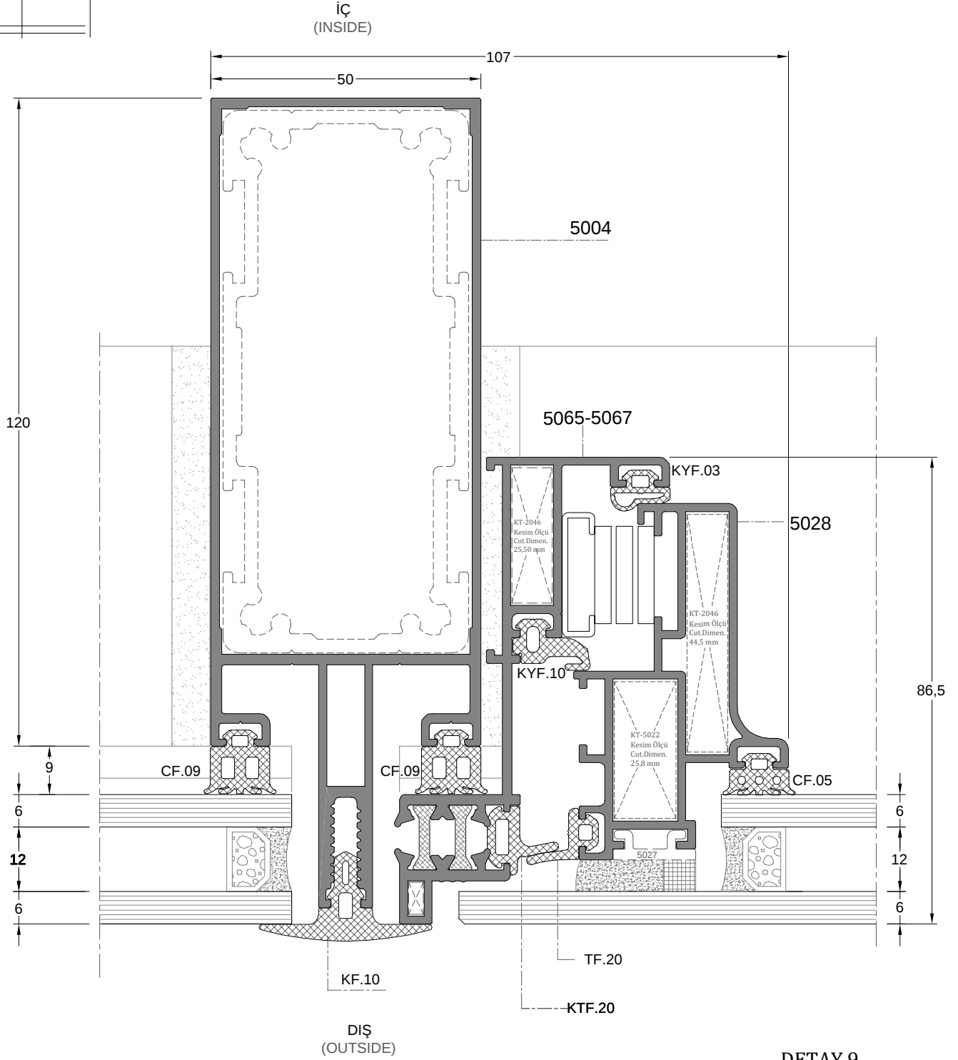
DETAY 9 DETAIL 9
