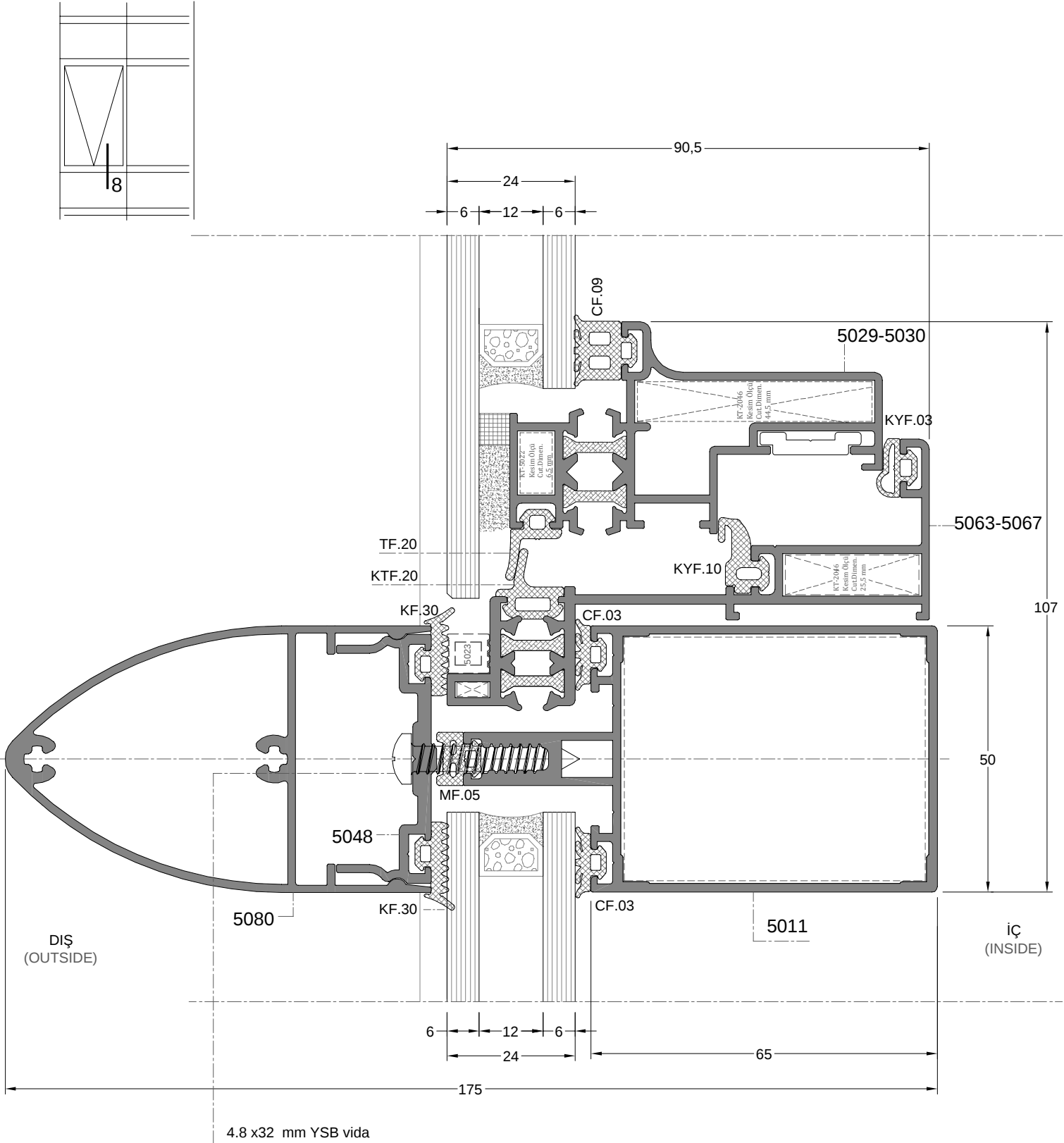
DETAY 8 DETAIL 8
