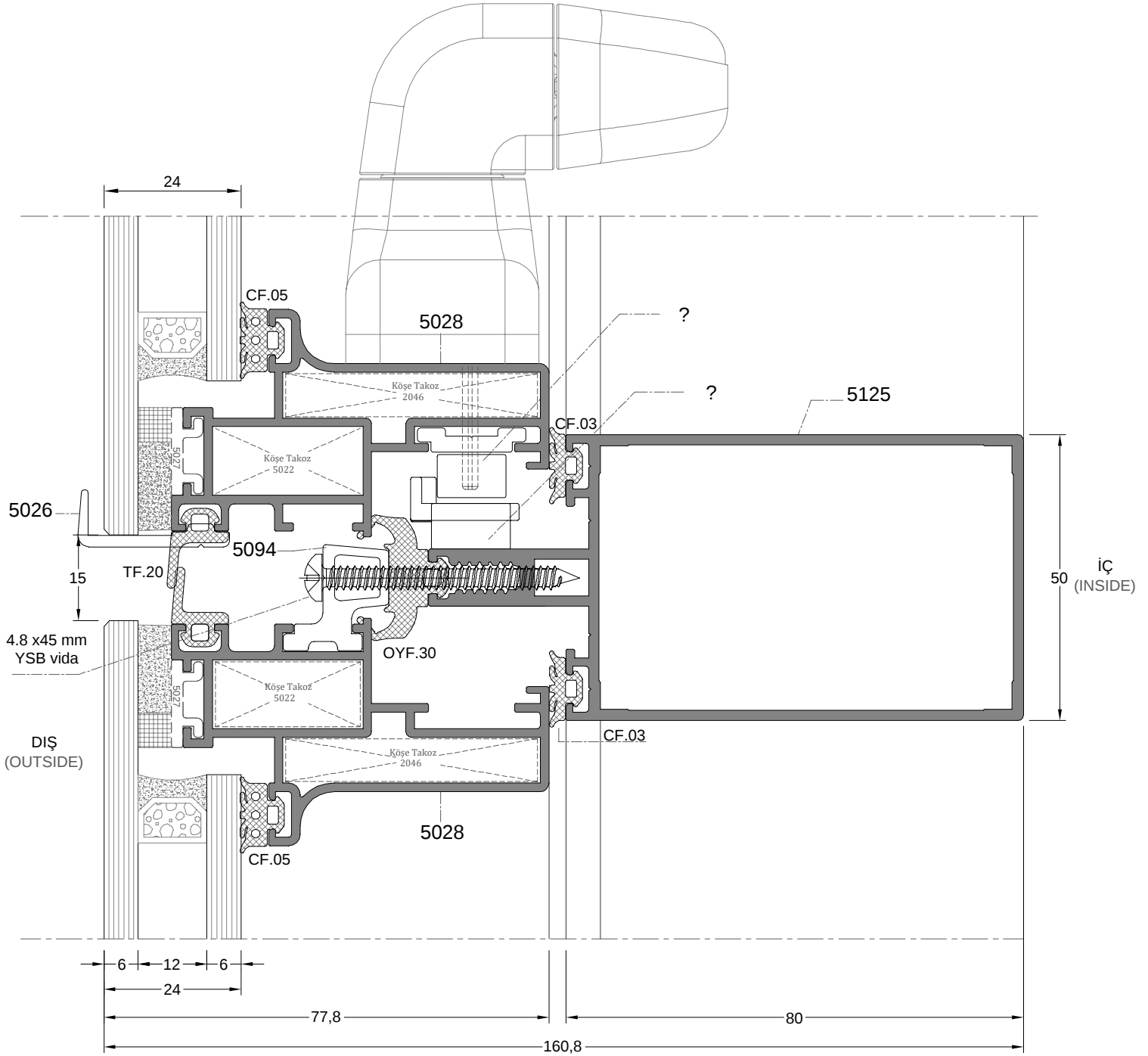
DETAY 2 DETAIL 2
