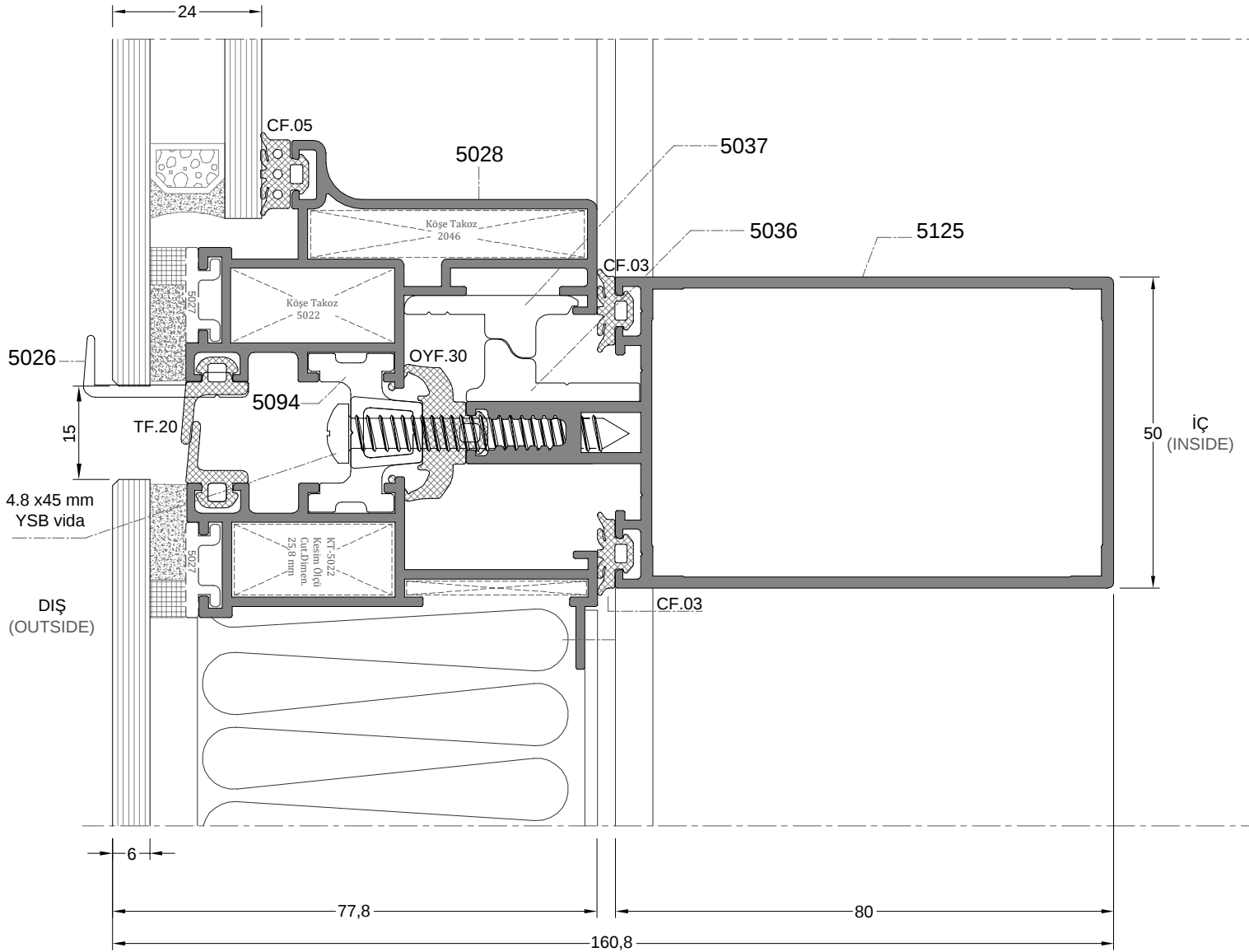
DETAY 4 DETAIL 4
