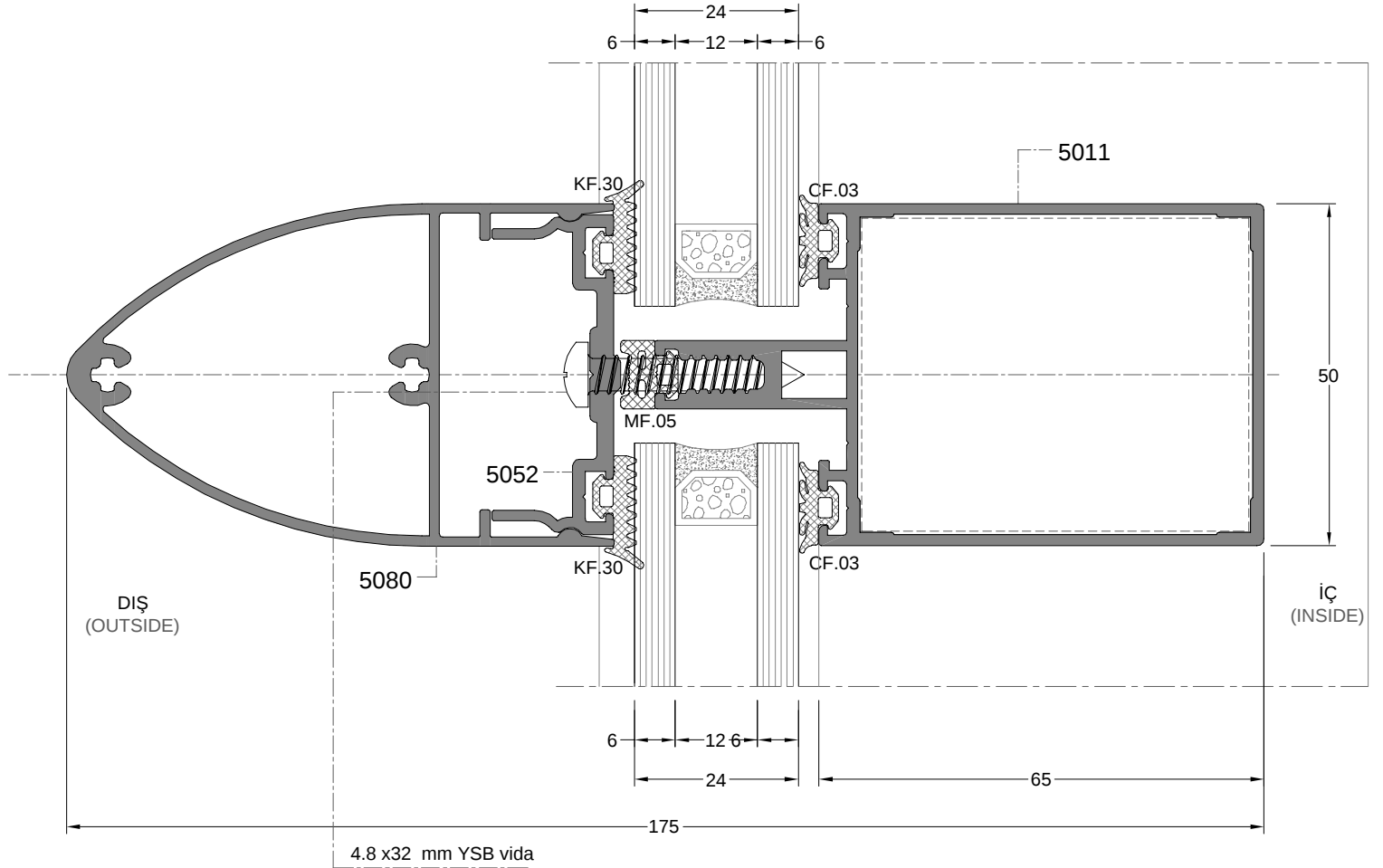
DETAY 2 DETAIL 2
