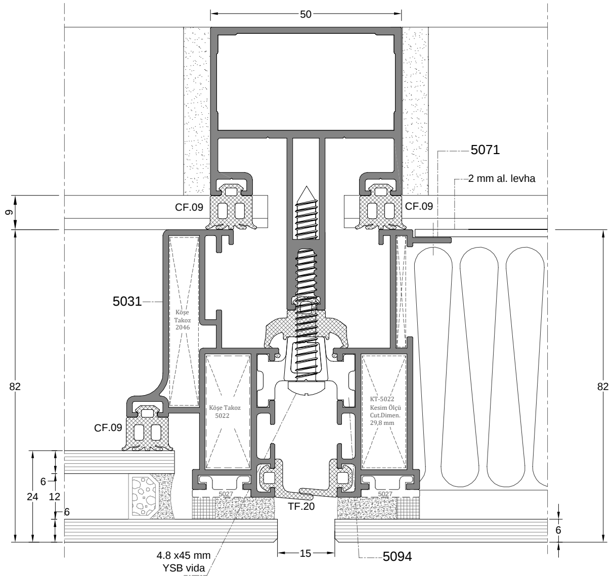
DETAY 4 DETAIL 4
