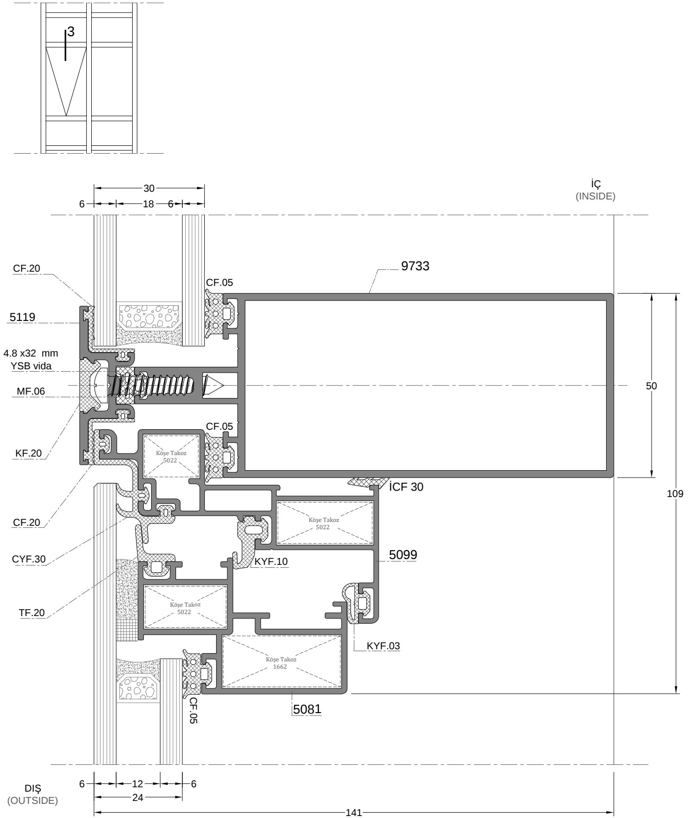
DETAY 3 DETAIL 3
