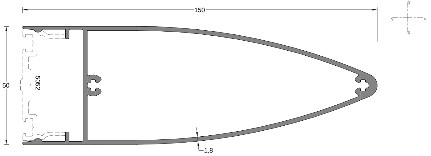
Badem Kapak Profili Almond Cover Profile
