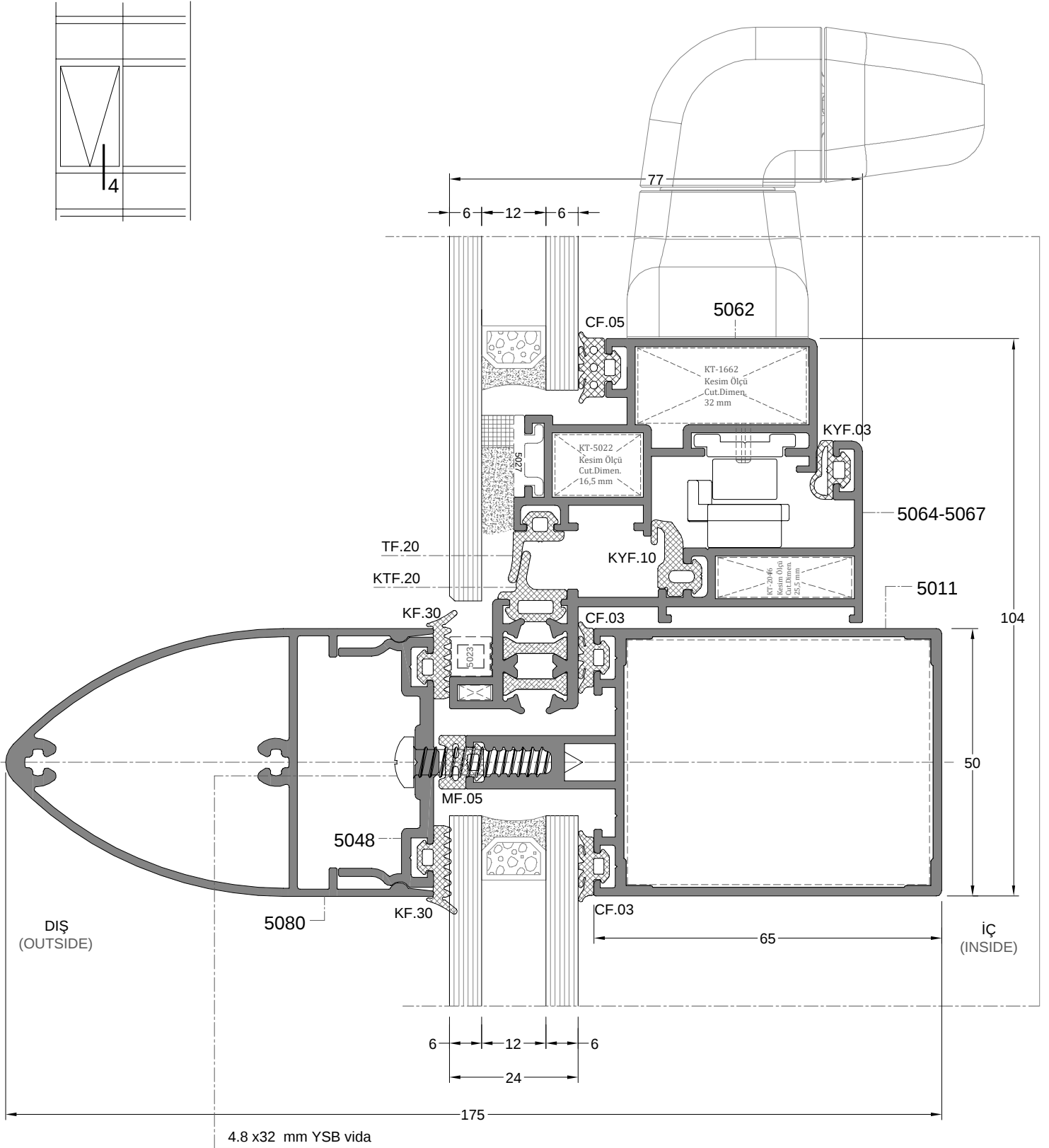
DETAY 4 DETAIL 4
