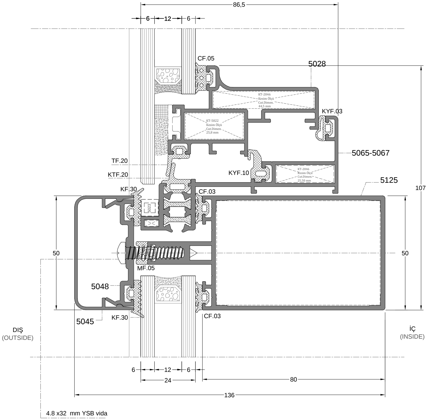
DETAY 10 DETAIL 10
