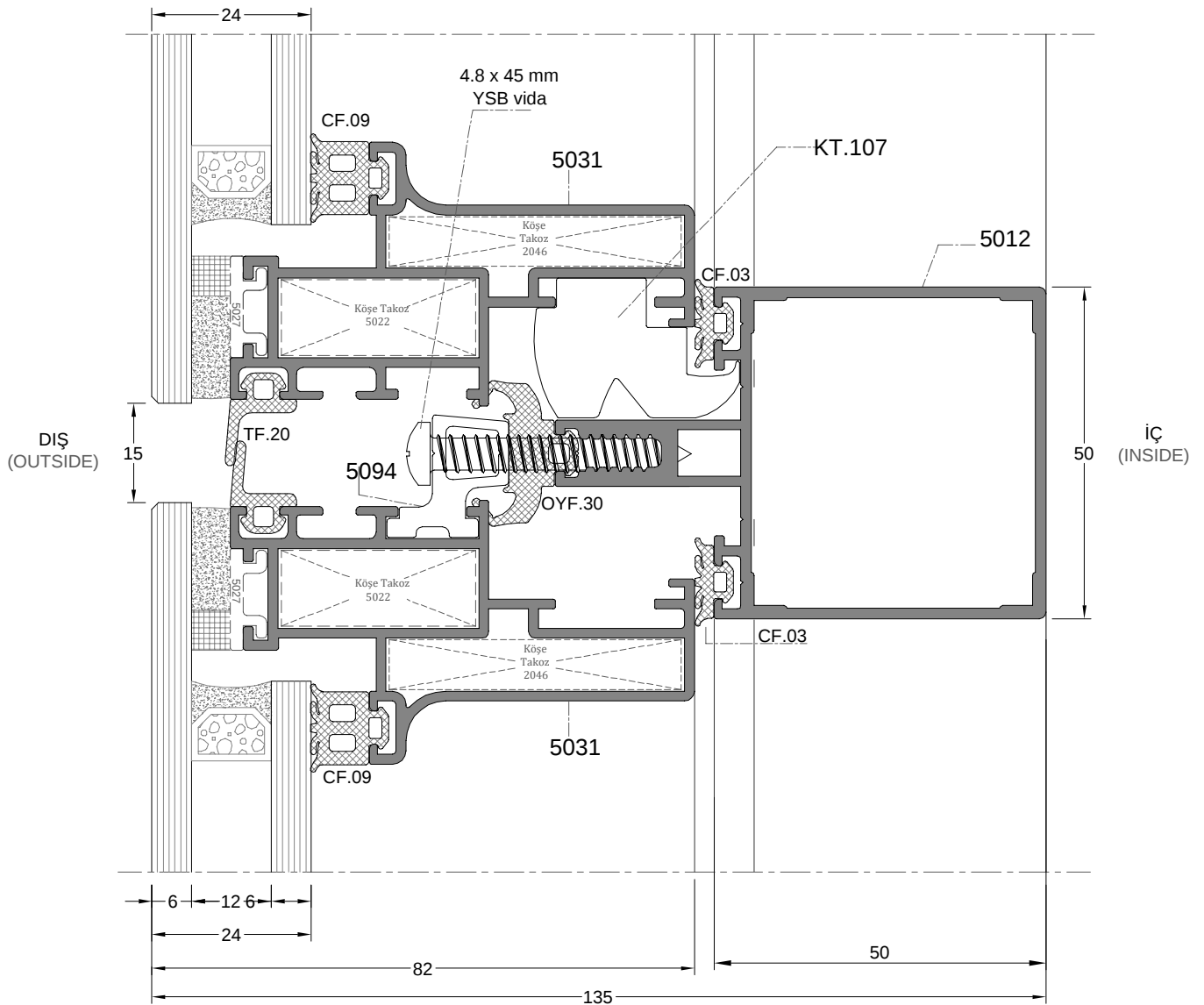
DETAY 3 DETAIL 3
