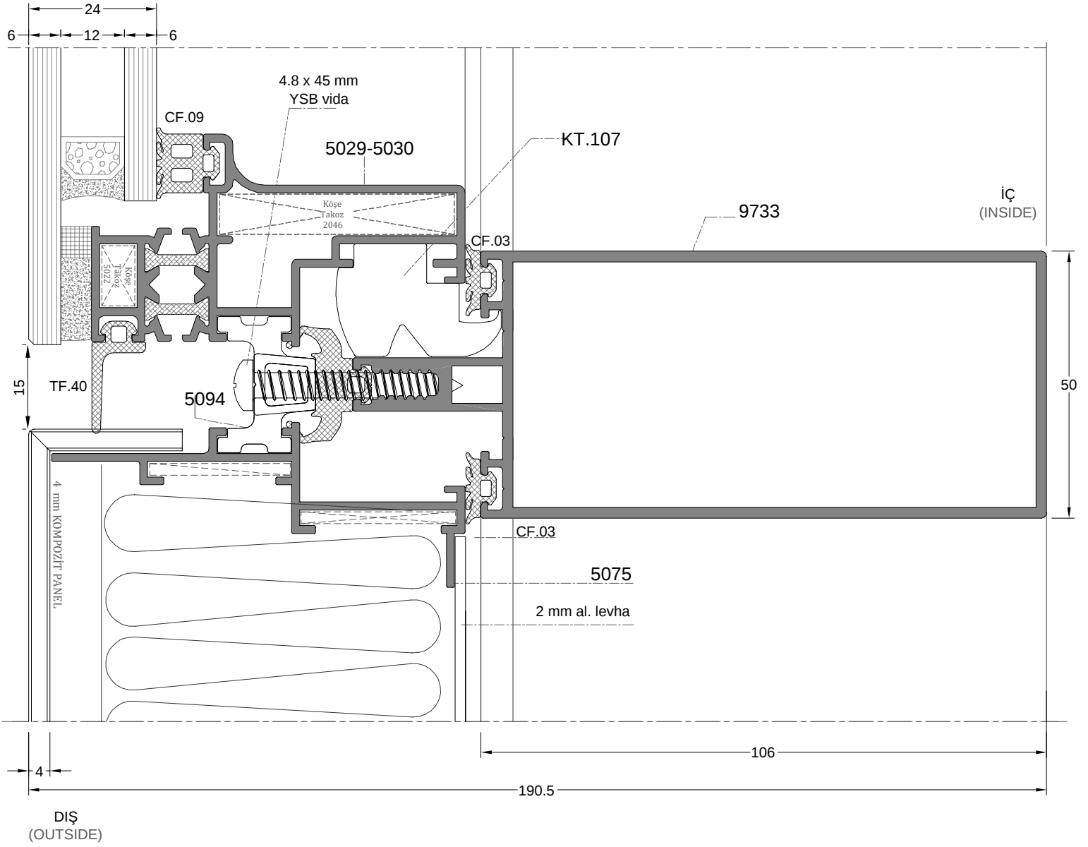
DETAY 6 DETAIL 6
