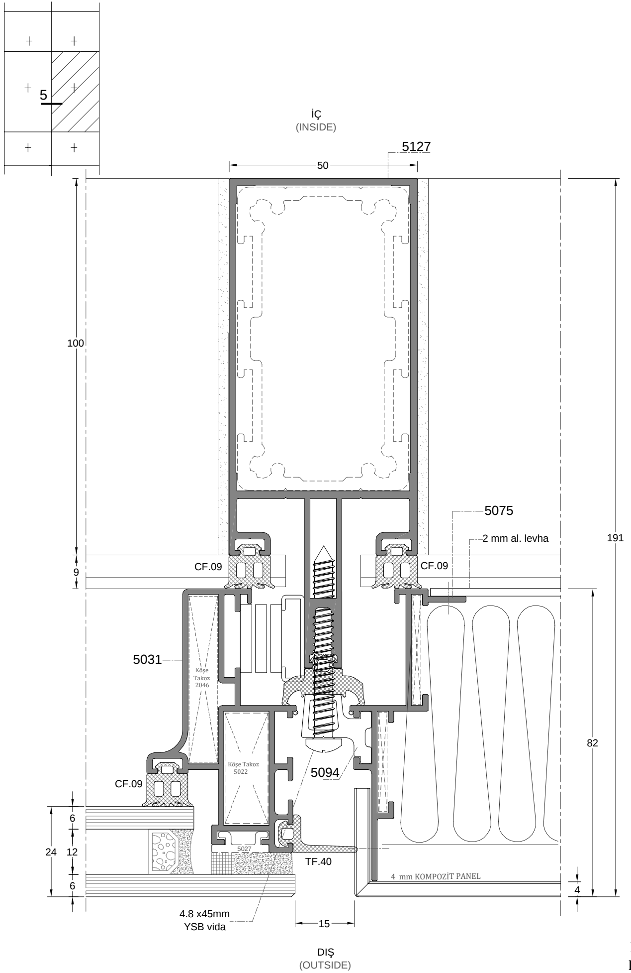
DETAY 5 DETAIL 5
