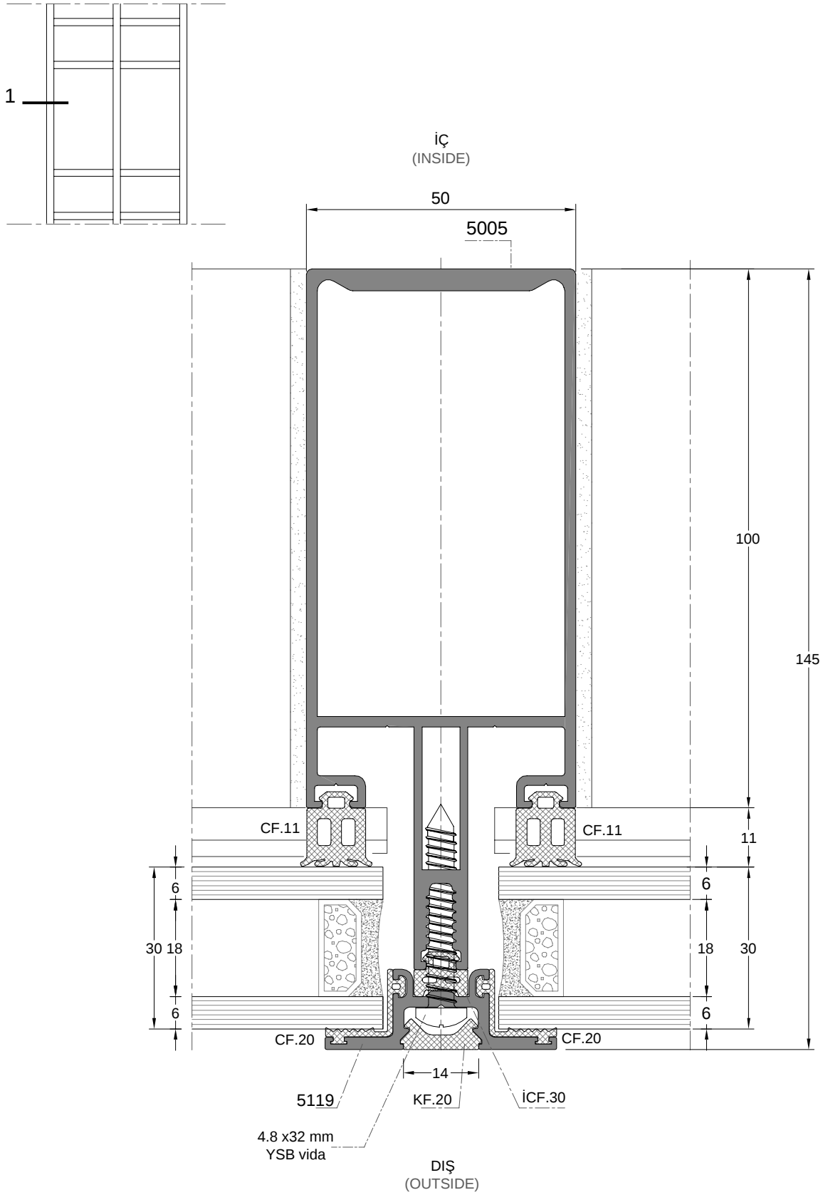
DETAY 1 DETAIL 1
