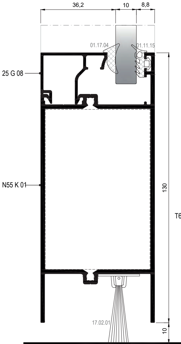
17 DETAYI DETAIL
