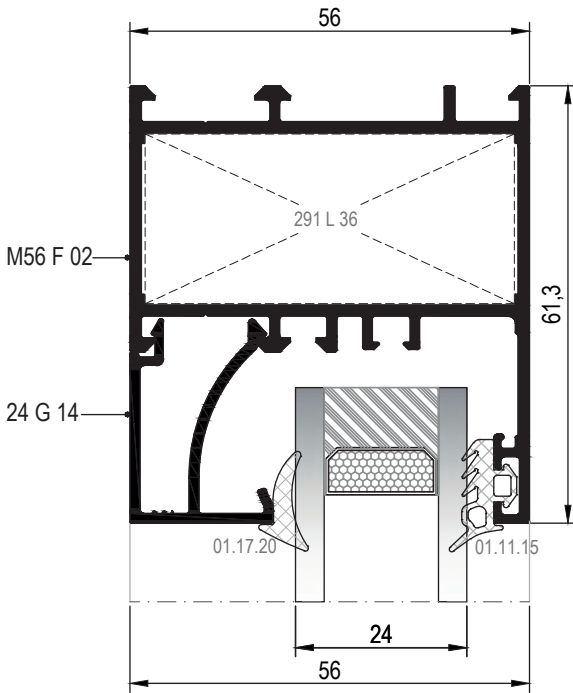
28 DETAYI DETAIL
