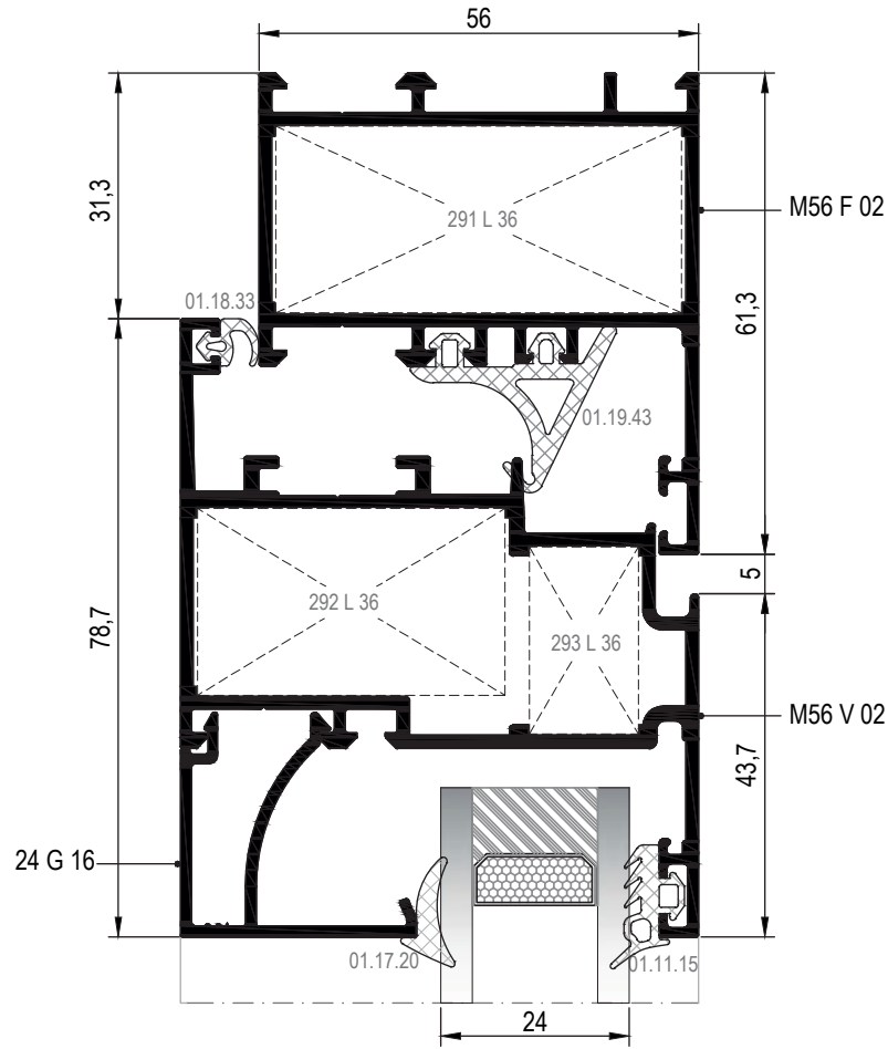
⑤ DETAYI DETAIL
