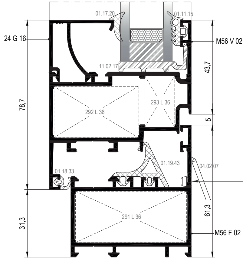
⑥ DETAYI DETAIL
