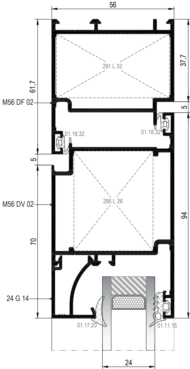
33 DETAYI DETAIL
