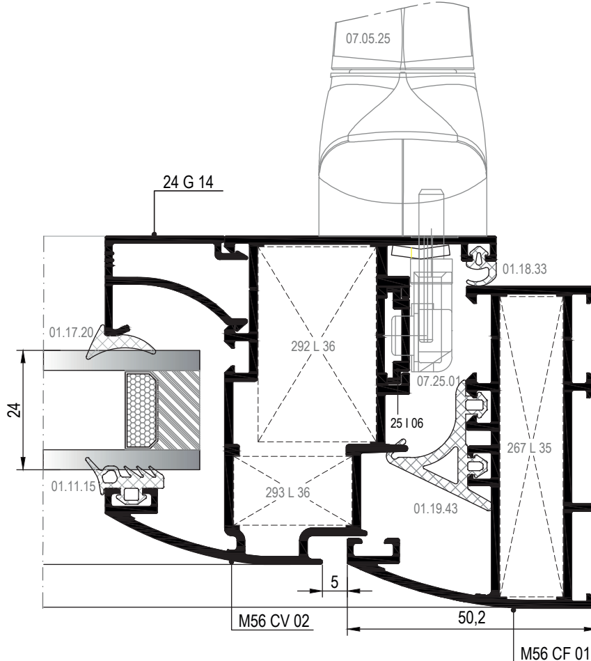
16 DETAYI DETAIL
