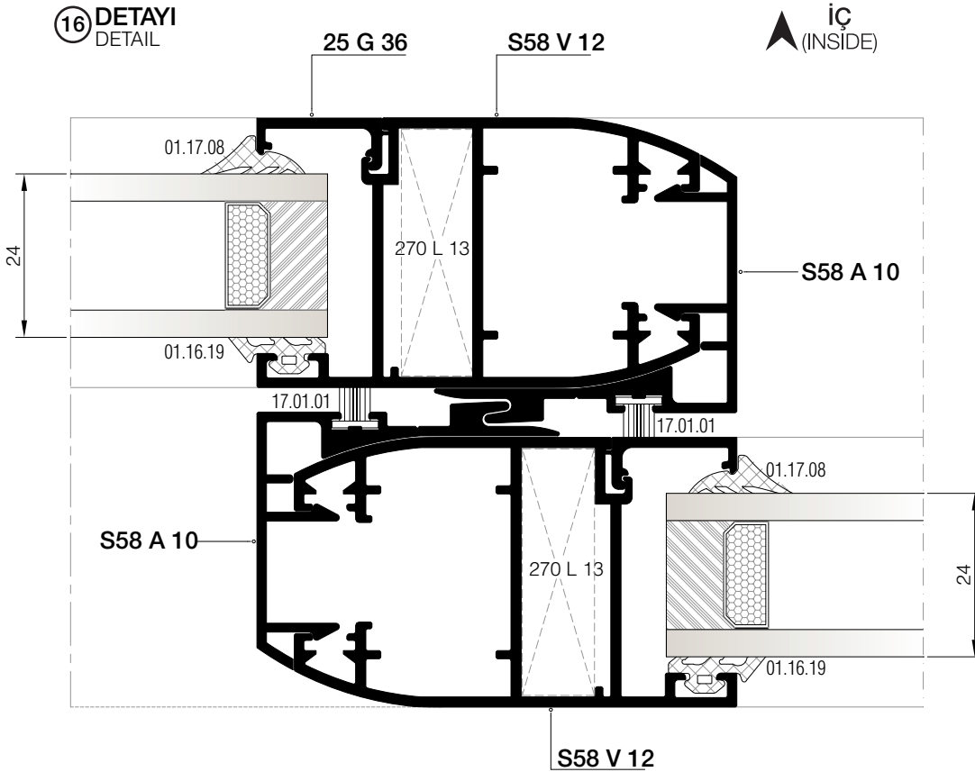
17 DETAYI DETAIL
