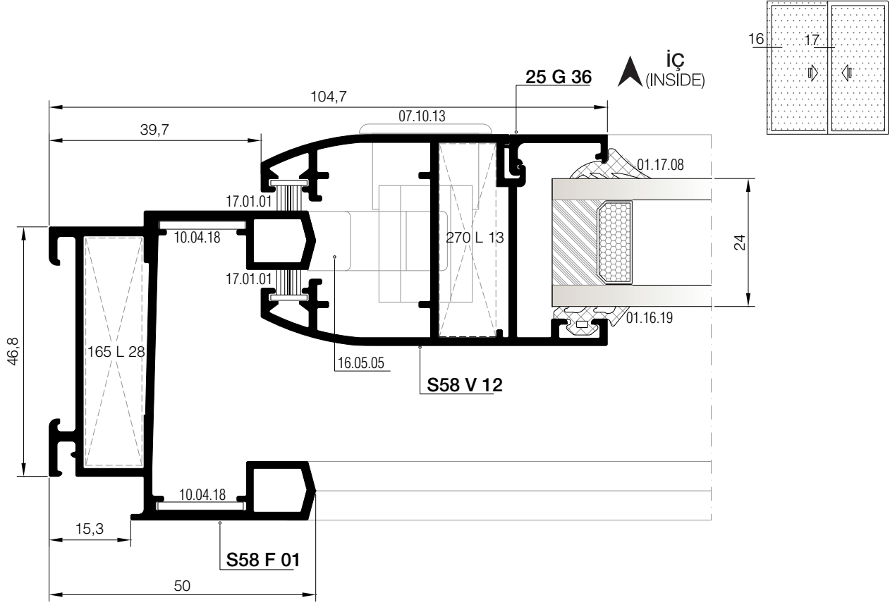
16 DETAYI DETAIL
