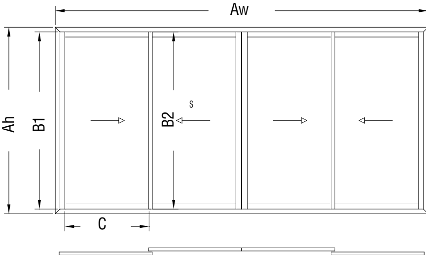
PROFİLLER / PROFILES
