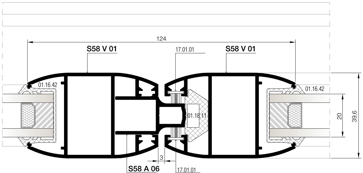
4 DETAYI DETAIL
