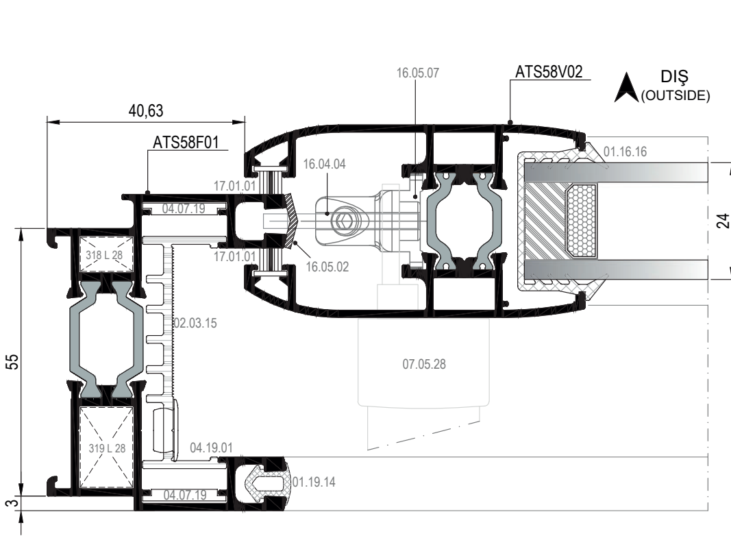
1A DETAYI DETAIL
