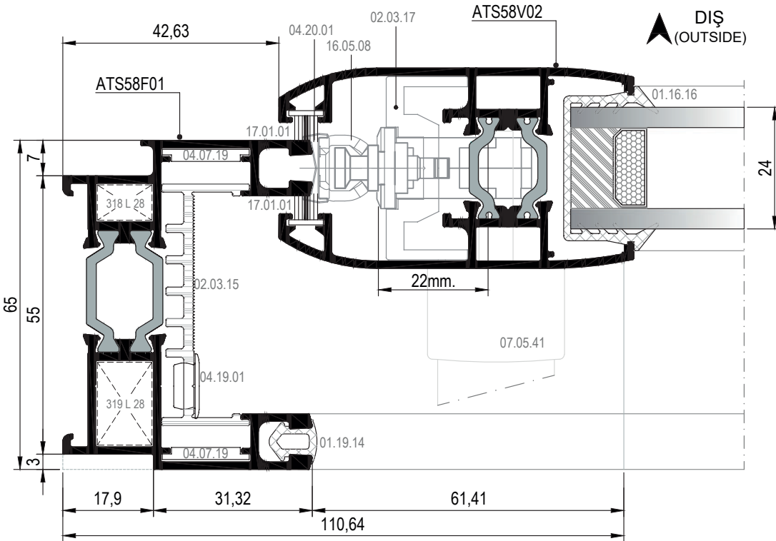
1B DETAYI DETAIL
