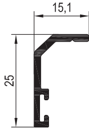
DAMLALIK PROFİLİ RAINDROP PROFILE
