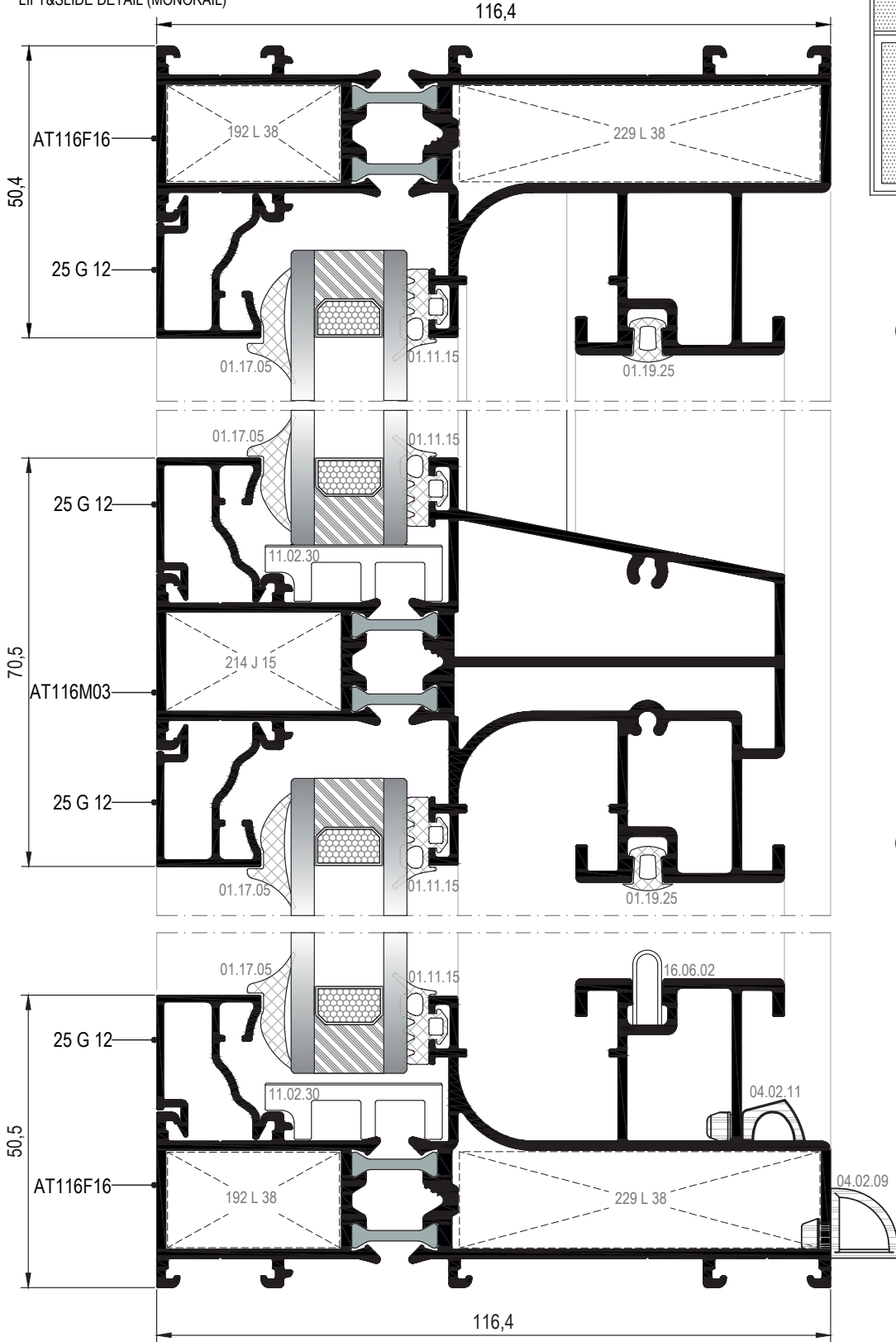
KALDIR SÜR DETAYI (MONORAY) LIFT&SLIDE DETAIL (MONORAIL)
