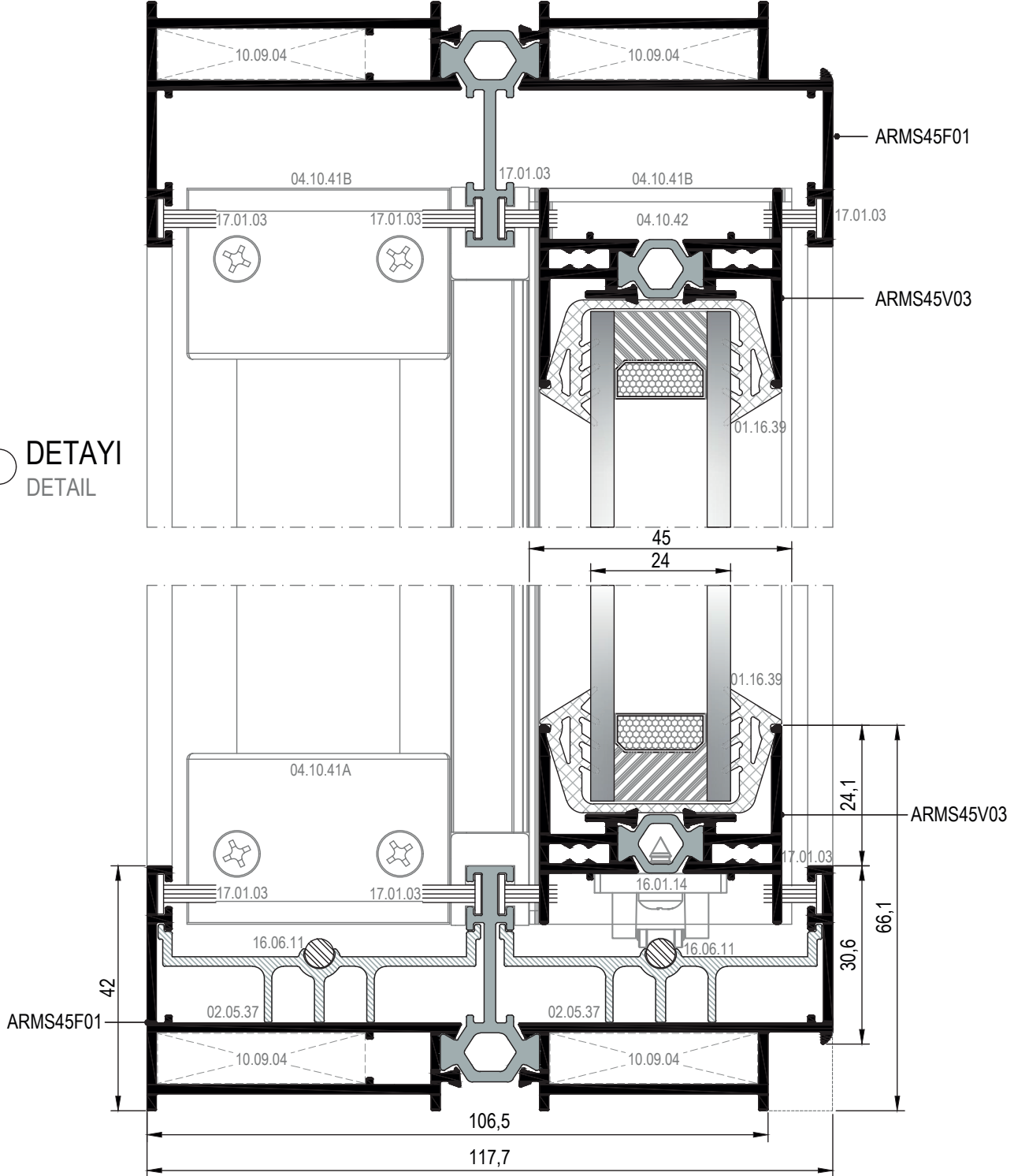
② DETAYI DETAIL
